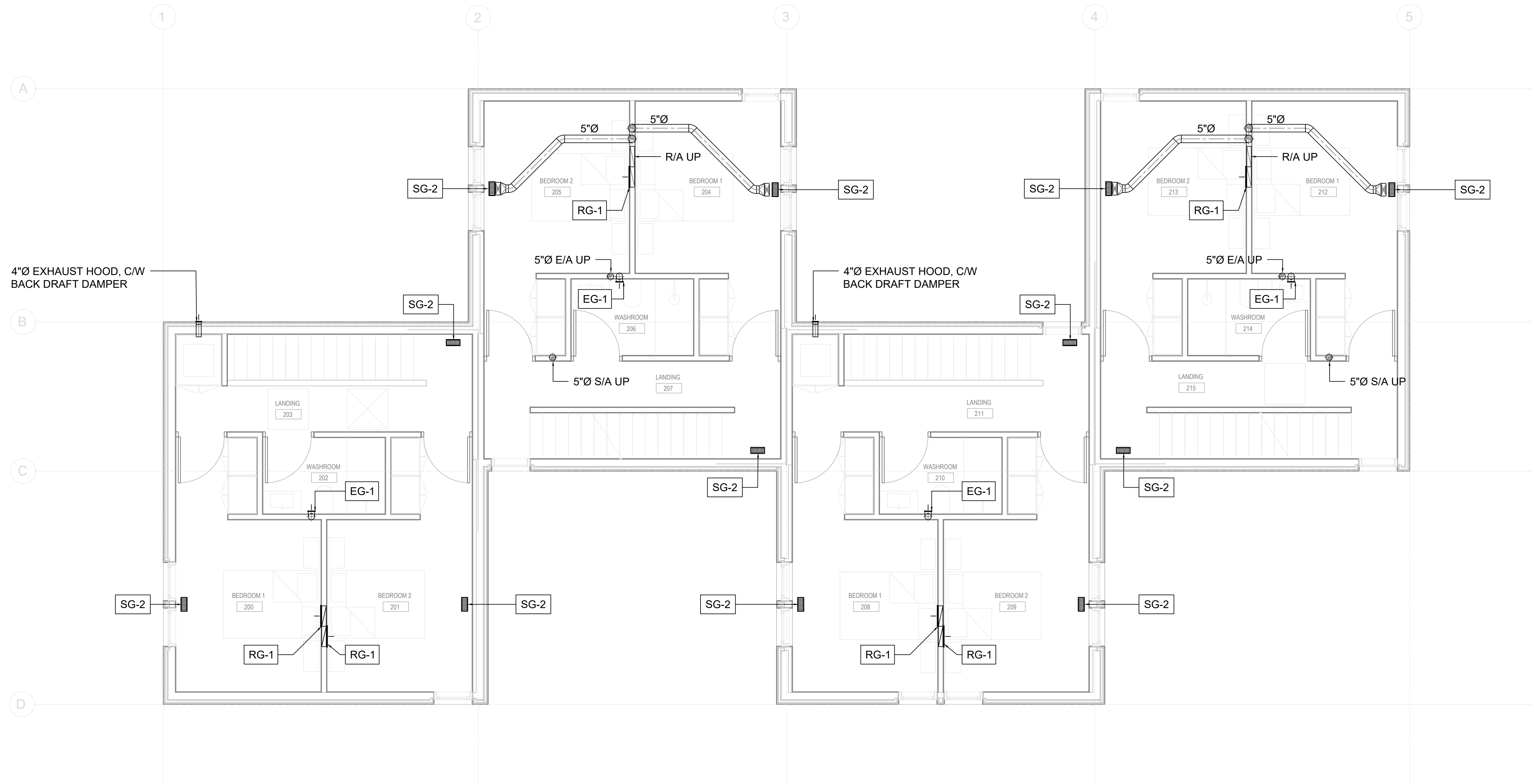
M2 LEVEL 2 FLOOR PLAN 1/4" : 1'
